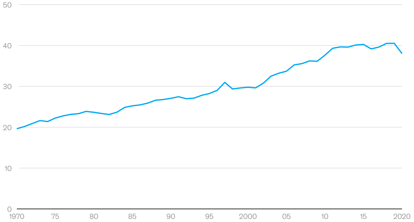
Annual global CO 2 emissions Billion metric tons per year
