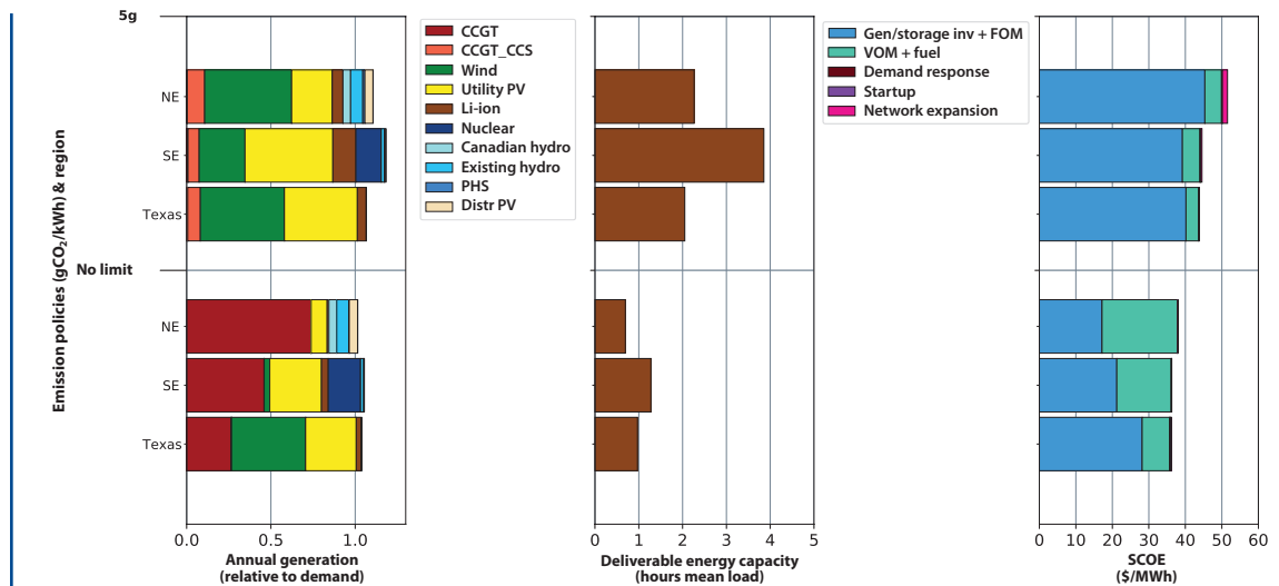
Figure ES.3: Annual generation relative to demand
