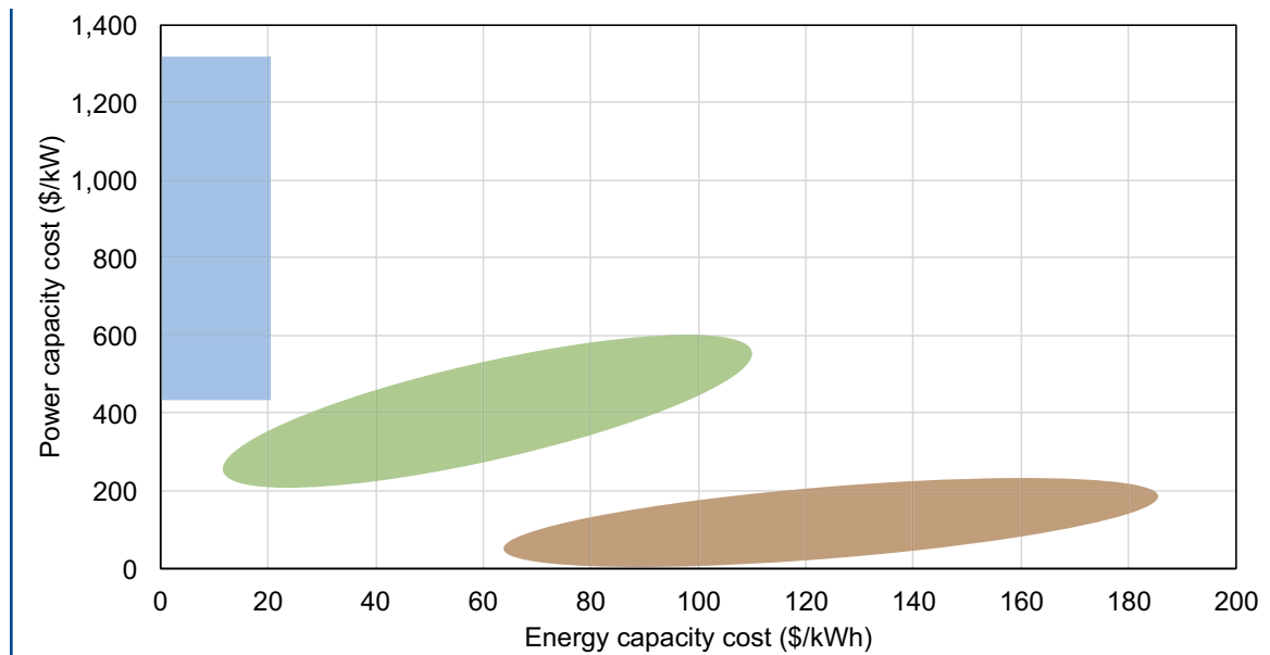
Figure 1.6 Three groups of storage technologies based on power- and energy-capacity costs
