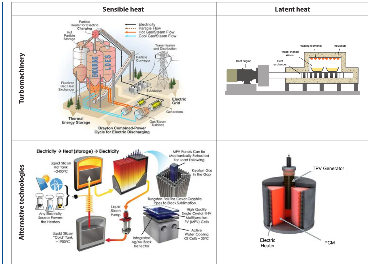
Clockwise from top left: particle storage with combined cycle (National Renewable Energy Laboratory 2018), silicon PCM in container atop a heat exchanger with Brayton turbine (Taylor, et al. 2020), silicon PCM with TPV (Datas, et al. 2016), liquid silicon with TPV (Amy, Seyf, et al. 2018).
