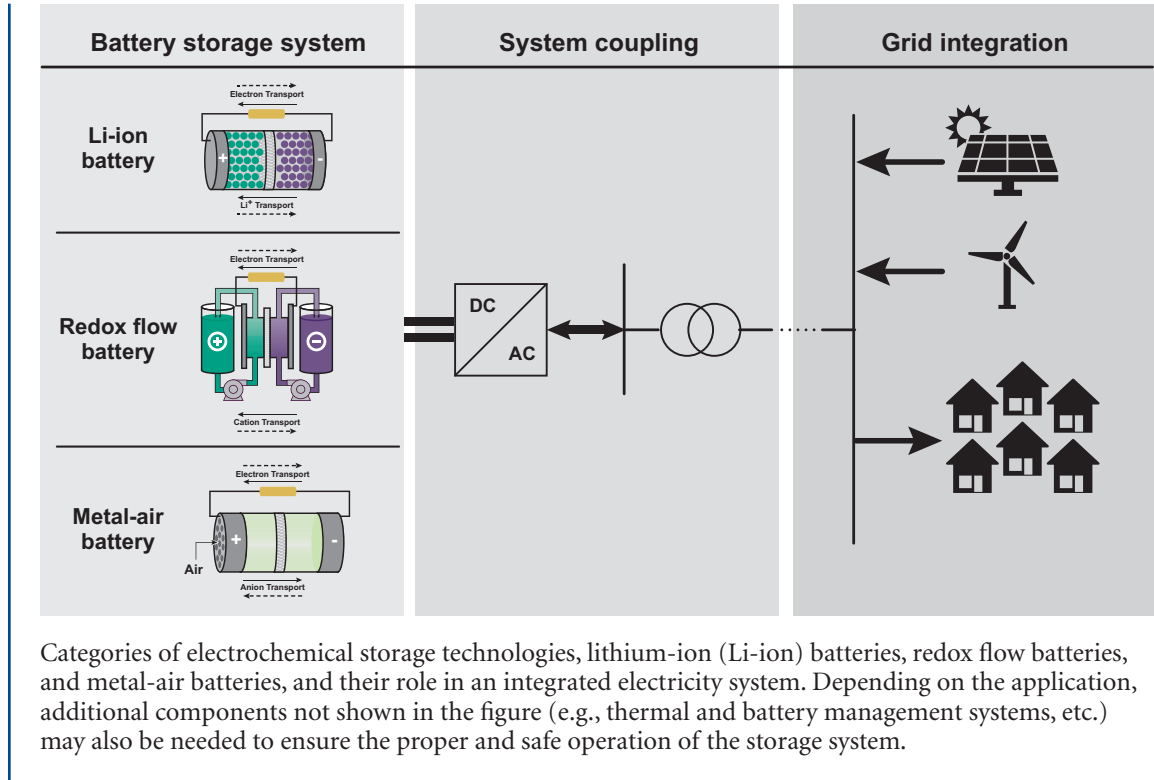
Figure 2.1 Categories of electrochemical storage technologies
