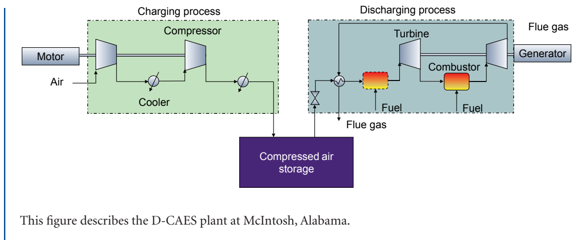
Figure 3.6 Flowsheet of a diabatic CAES system with a recuperator
