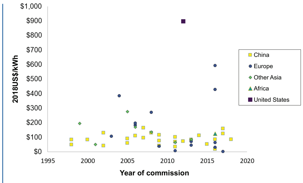
Figure 3.3 Capital cost per kWh
