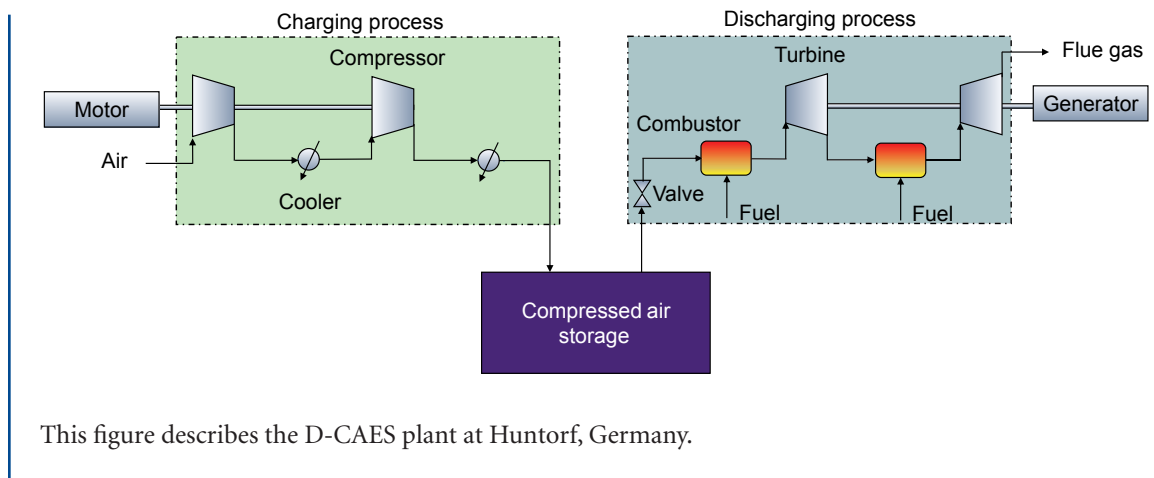
Figure 3.5 Flowsheet of a conventional diabatic CAES system with two combustors
