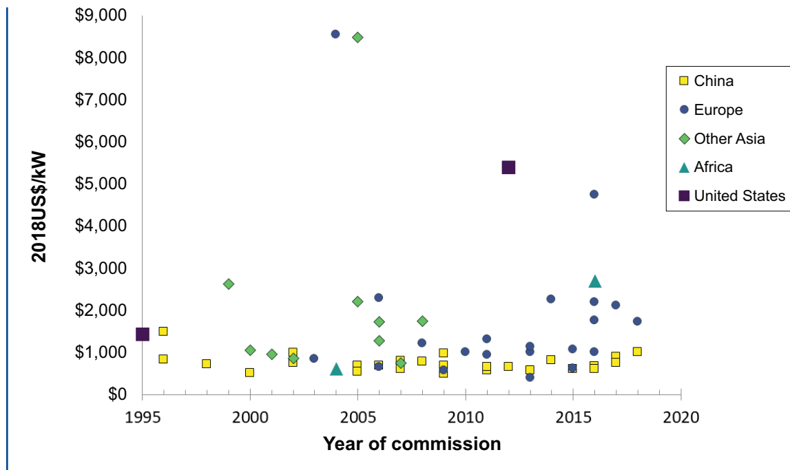
Figure 3.2 Capital cost per kW
