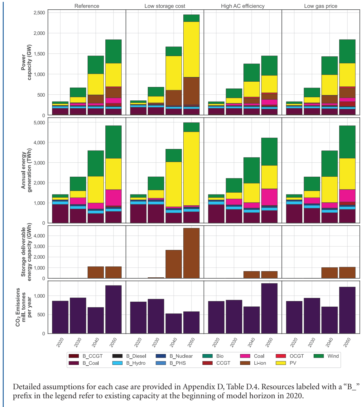
Figure 7.11 Installed capacity (1st row), annual energy generation (2nd row), storage energy capacity (3rd row), and annual CO 2 emissions (4th row) for reference case (1st column), as well as cases with alternative assumptions for battery storage capital cost (2nd column), high AC efficiency (3rd column), and gas prices (4th column)
