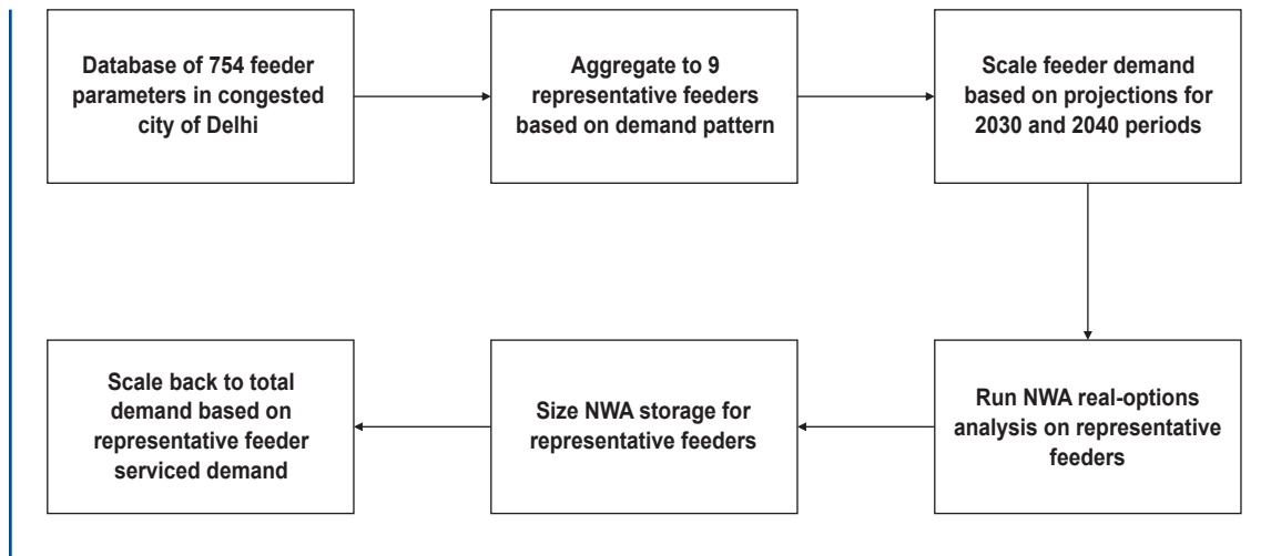
Figure 7.8 Approach for computing megacity-level DLS potential in the Indian context
