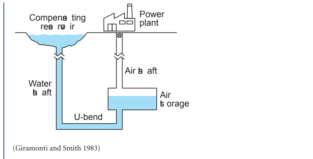
Figure 3.12 Surface reservoir provides pressure to enable air extraction at constant pressure
