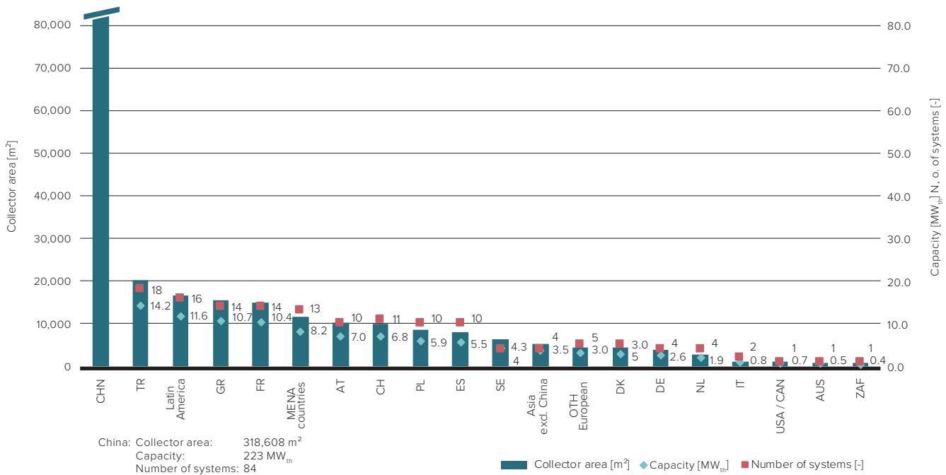
Large-scale systems for residential, public and commercial buildings Collector area, capacities installed and number of systems by country (2021)
